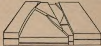
FIG. 476. — Schematic representation of a "zone of diverse displacement" in the Great Basin of the western United States (after Powell).
